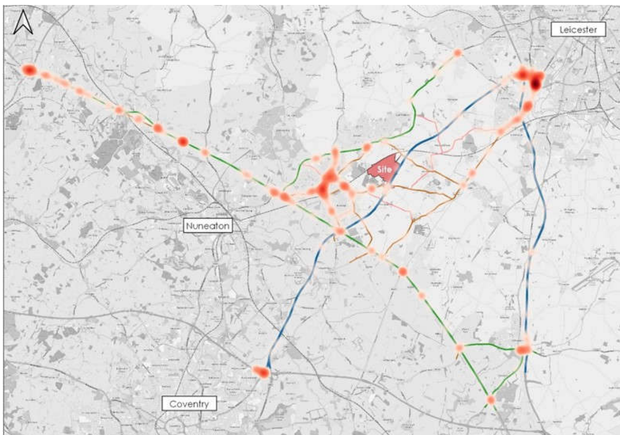
Figure 4-11: Collision Heatmap
